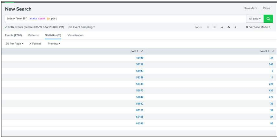
Figure 3-18.
