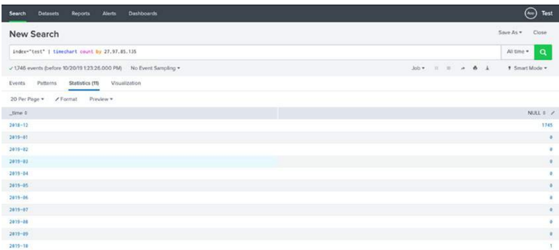
Figure 5-17.
