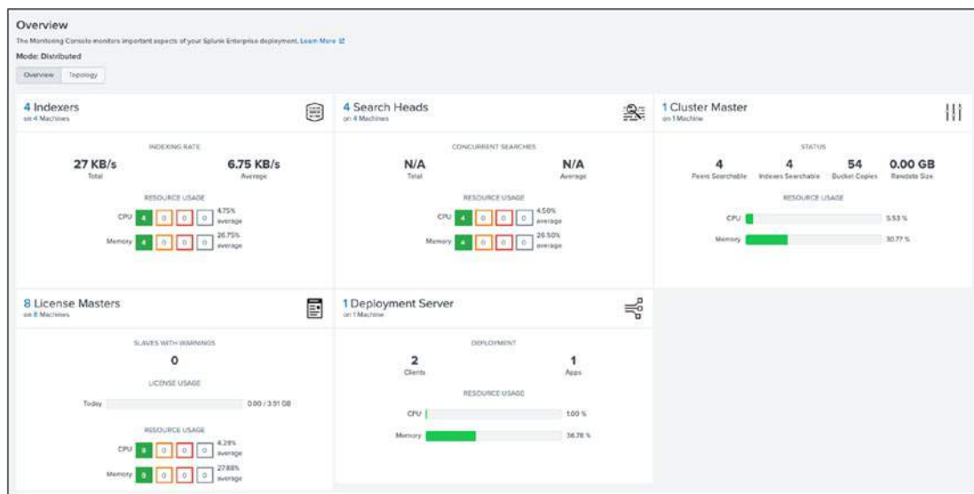
Figure 14-5. Monitoring Console:Deployment
