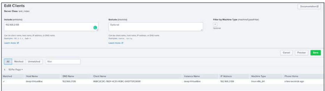
Figure 15-5. test_index:deployment clients
