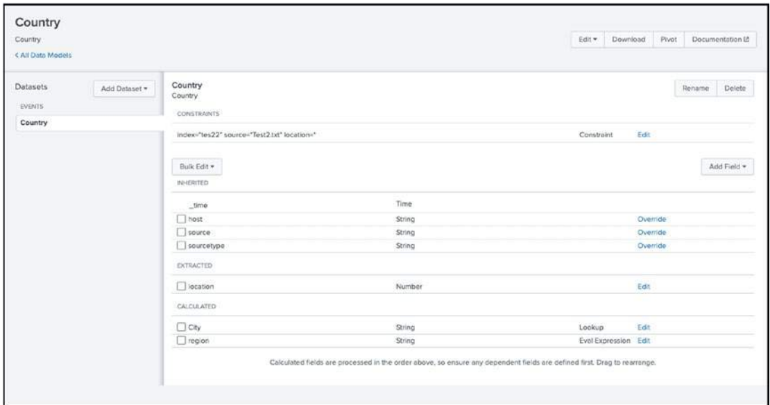
Figure 5-6. Dataset Country
