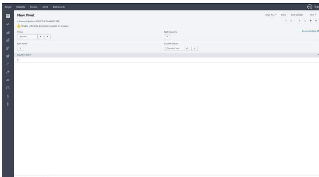
Figure 5-20.
