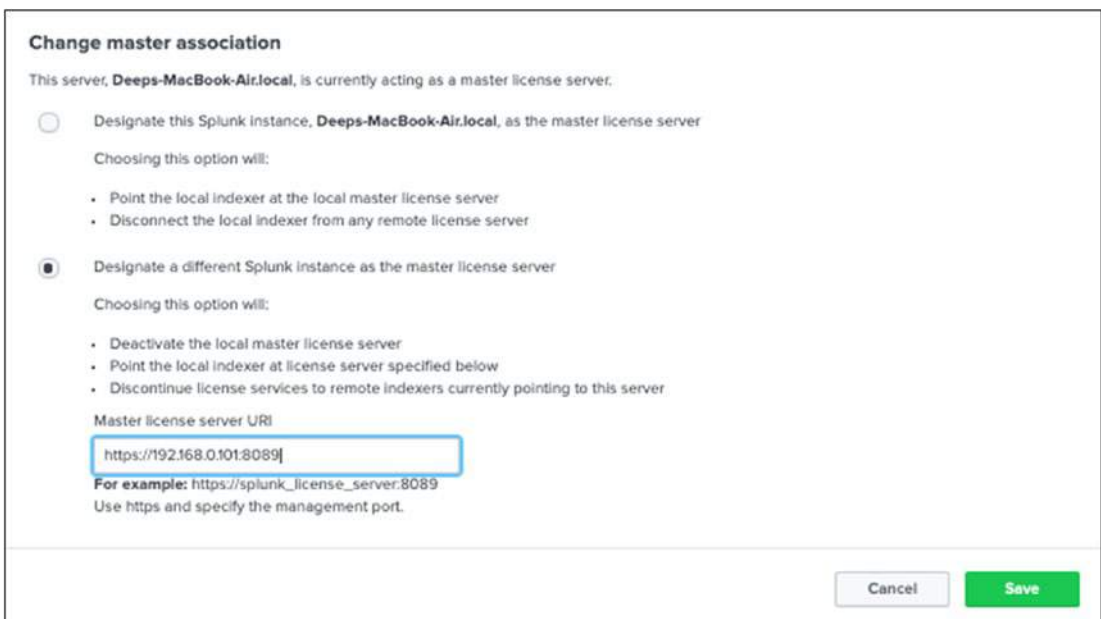
Figure 8-3. License Master
