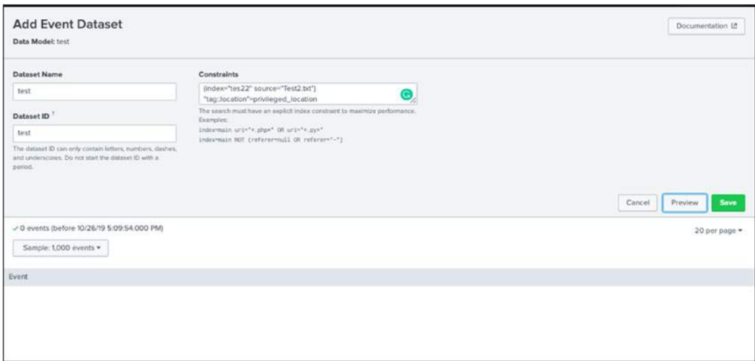
Figure 5-18.
