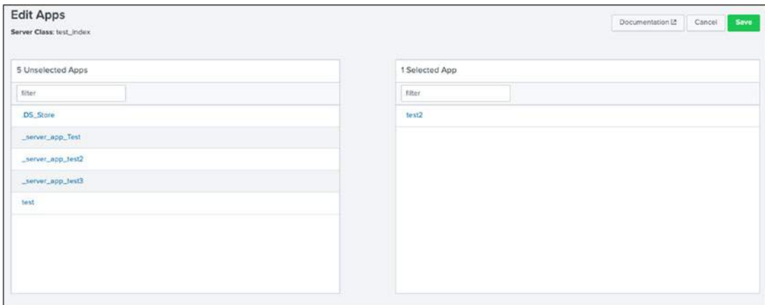
Figure 15-4. test_index:deployment apps
