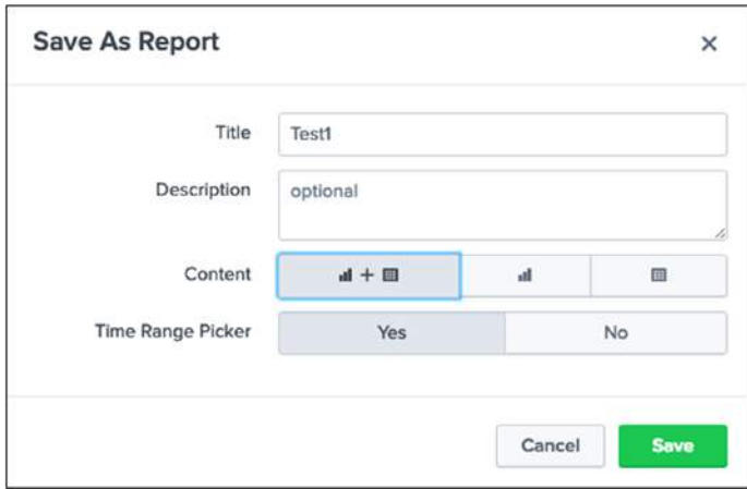
Figure 4-11. Splunk report
