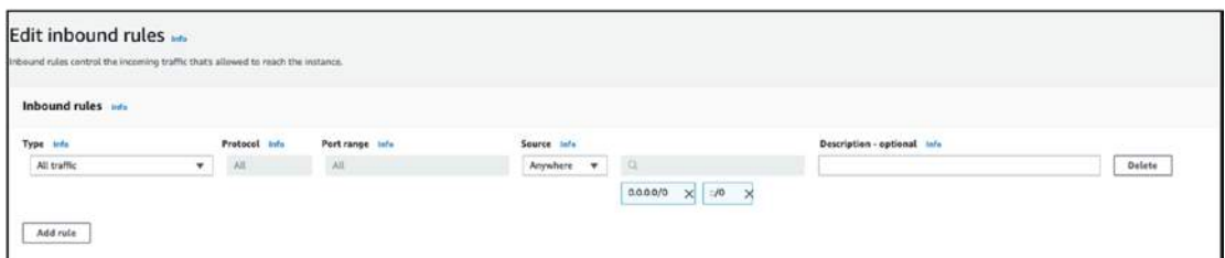
Figure 18-3. Security Group:Main
