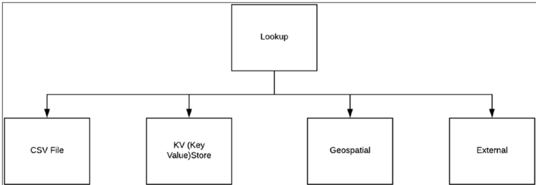
Figure 4-1. Splunk lookups
