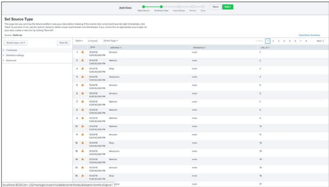
Figure 3-11. Sourcetype:test2
