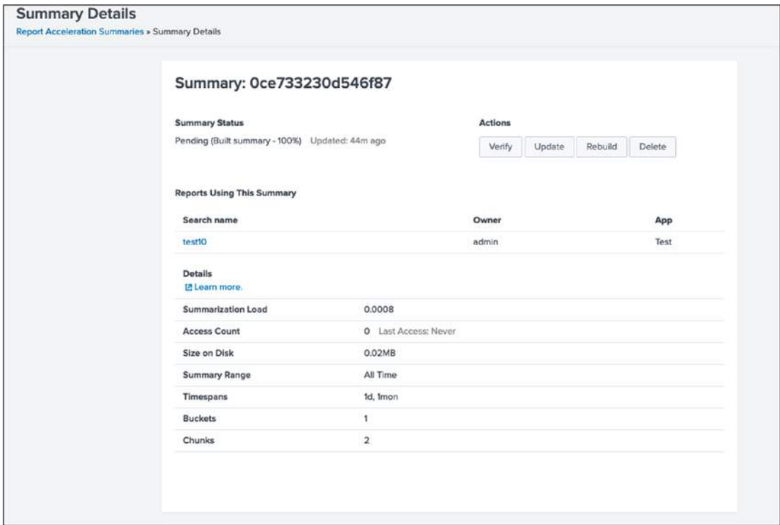
Figure 4-15. Sample summary
