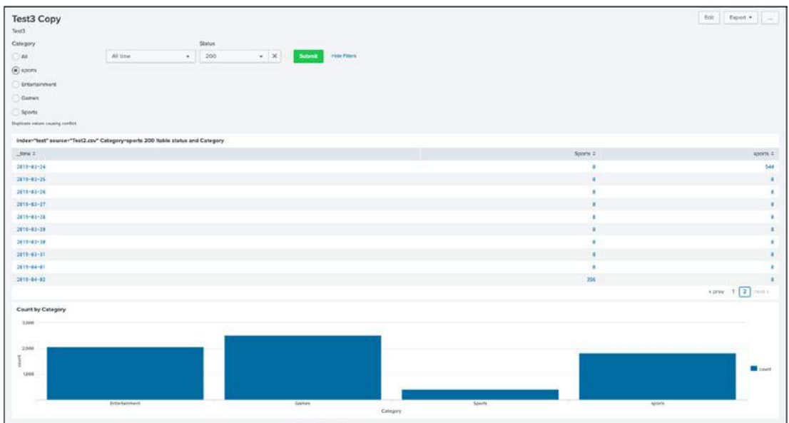
Figure 6-11.
