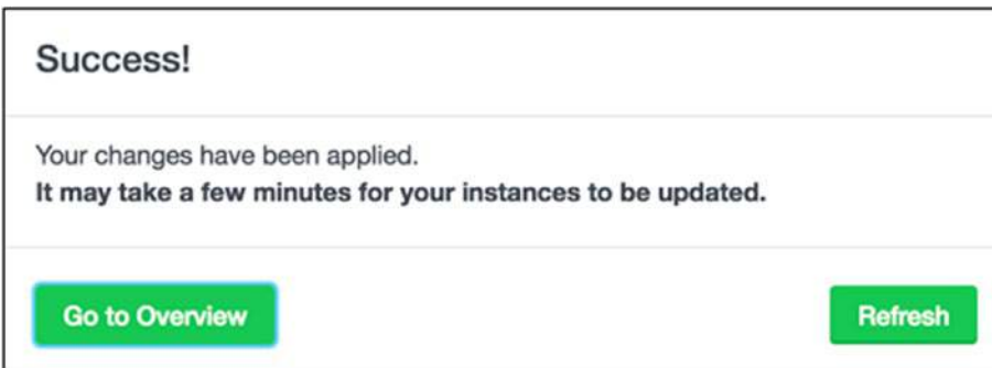
Figure 14-4.
