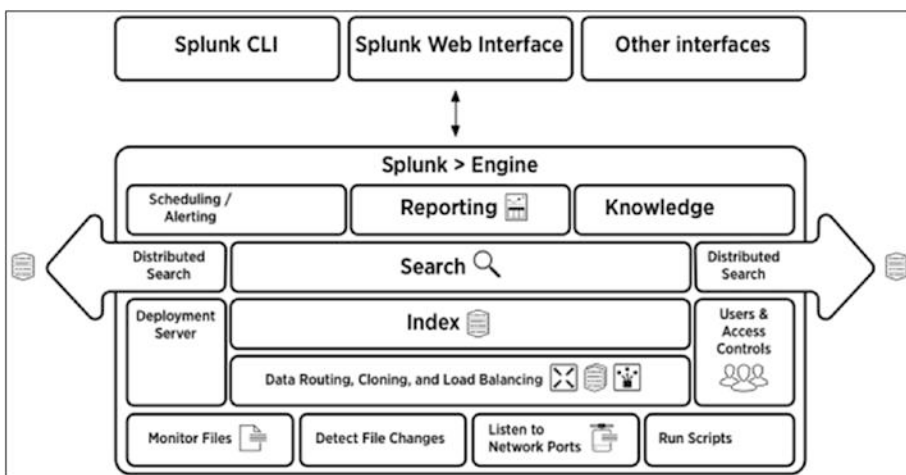
Figure 1-3. Splunk's architecture
