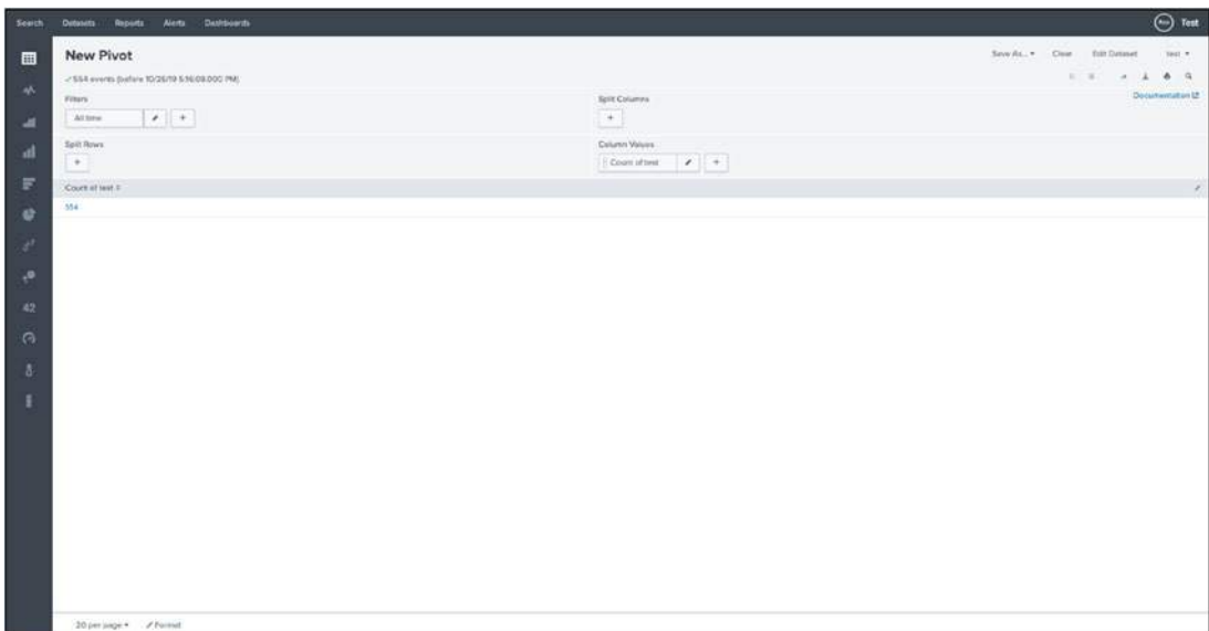
Figure 5-22.
