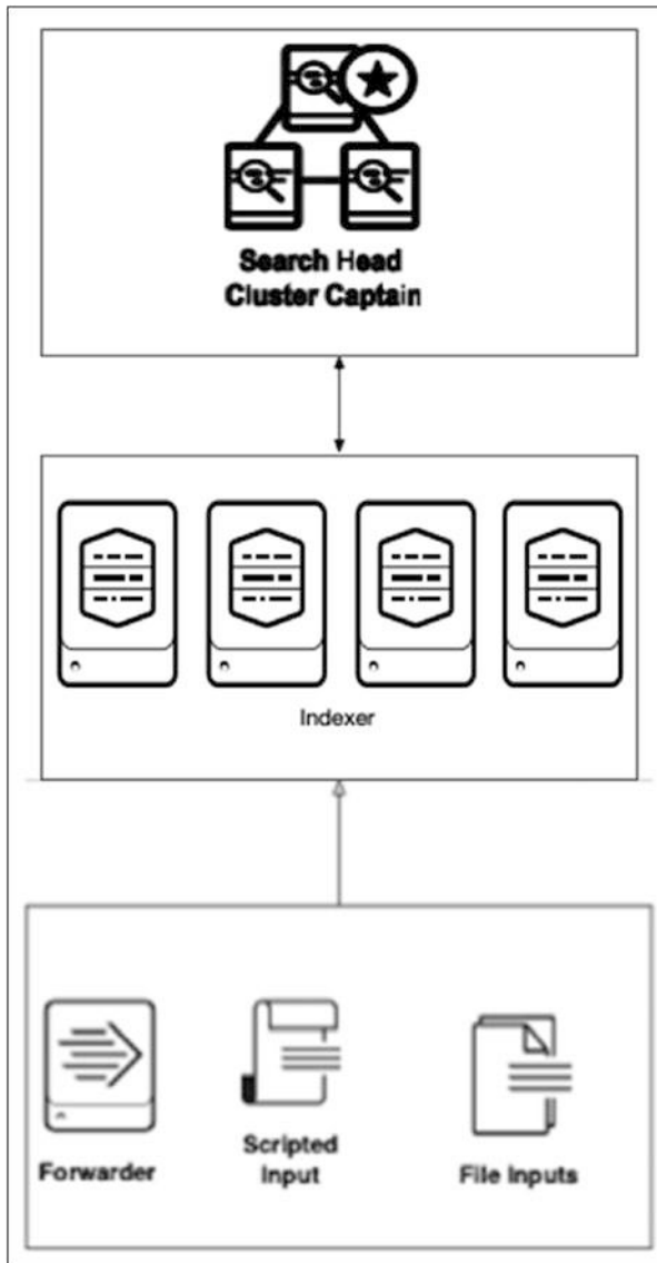
Figure 13-4. Search Head Clustering Constituent Architecture
