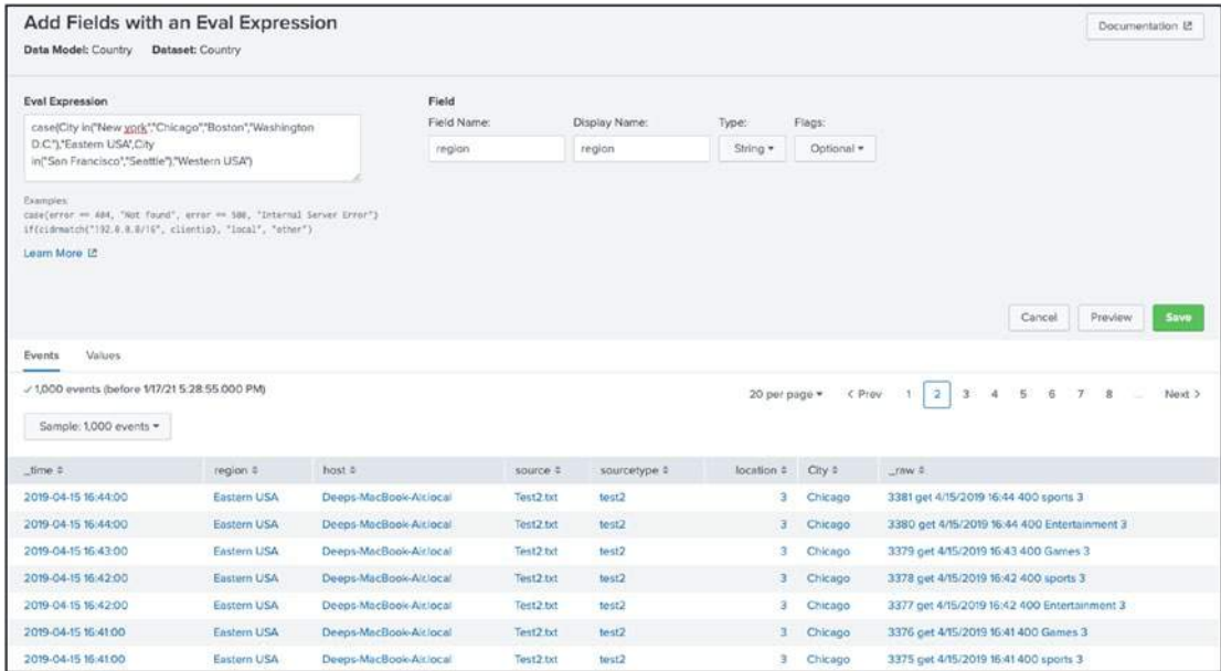
Figure 5-5. Evaluate Expression:region
