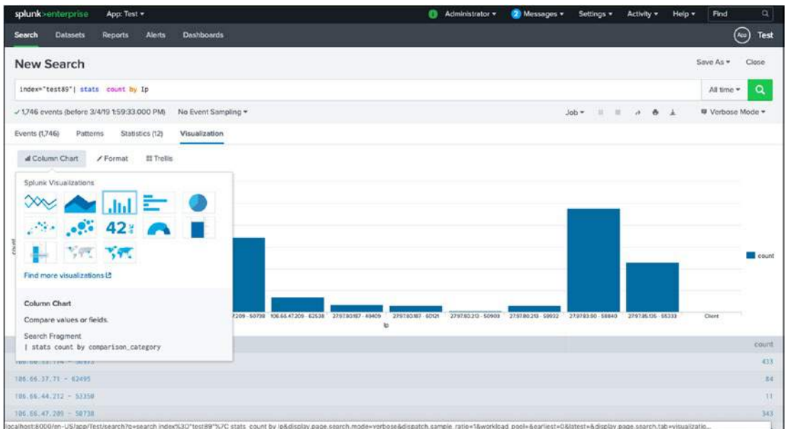
Figure 4-10. Splunk visualization
