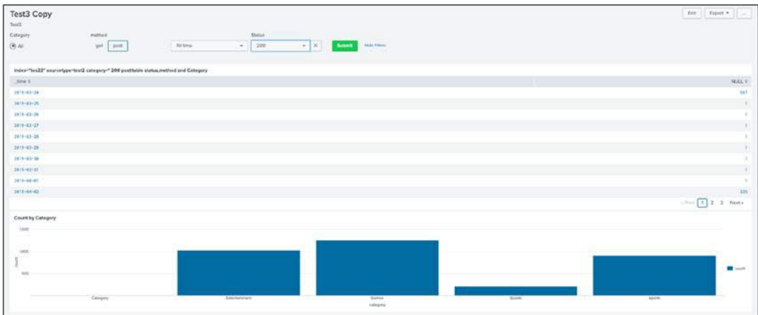
Figure 6-12.
