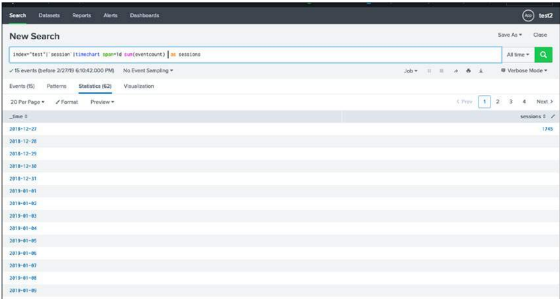
Figure 3-7. Macro's Output
