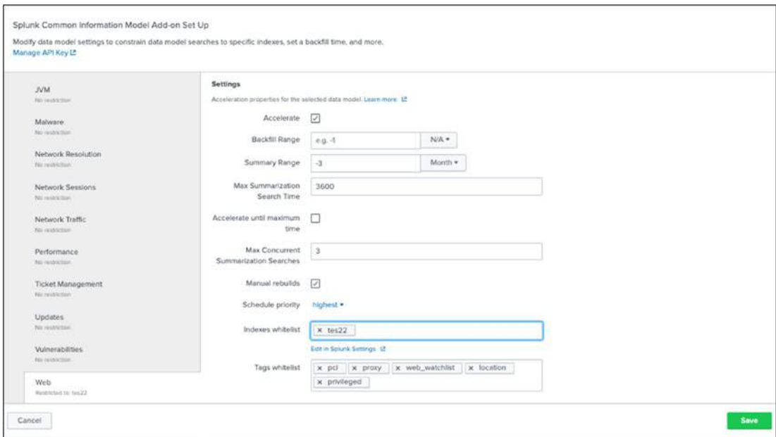
Figure 5-21.
