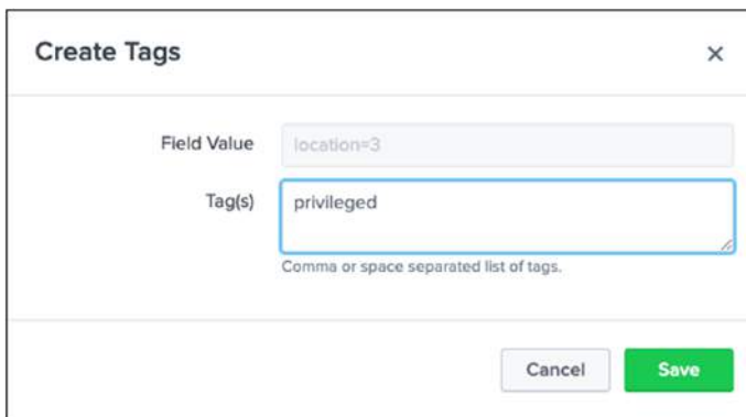
Figure 4-7. Splunk tags
