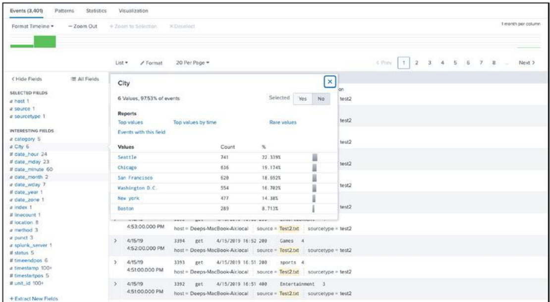
Figure 4-6. Splunk lookup
