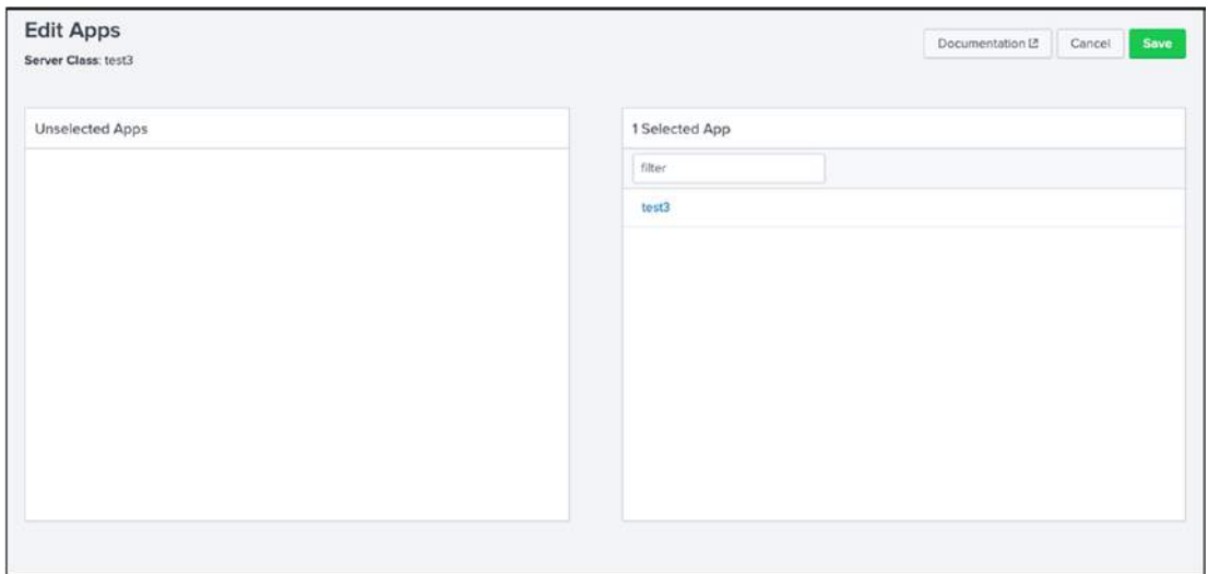
Figure 15-1. Forwarder Management
