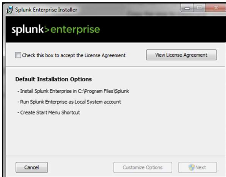
Figure 1-9. Installing Splunk
