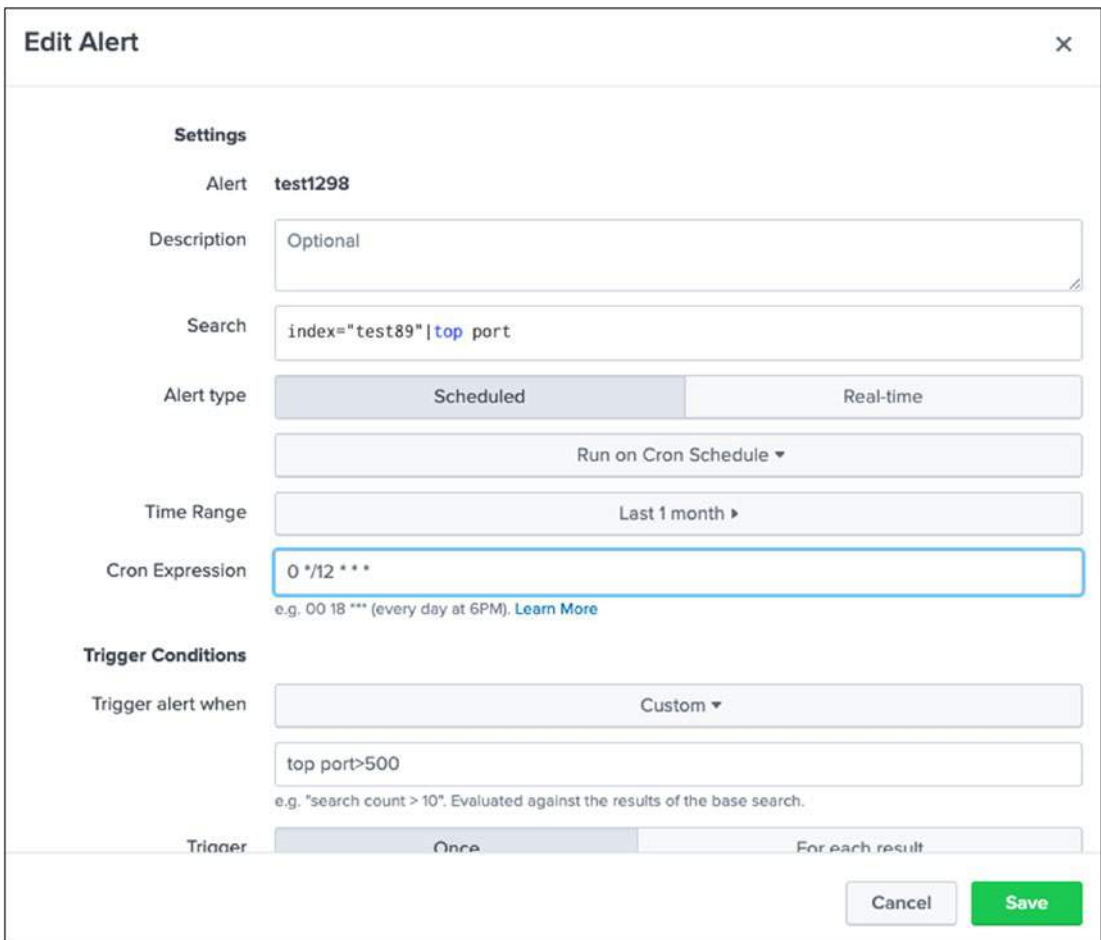
Figure 4-20. Cron expression
