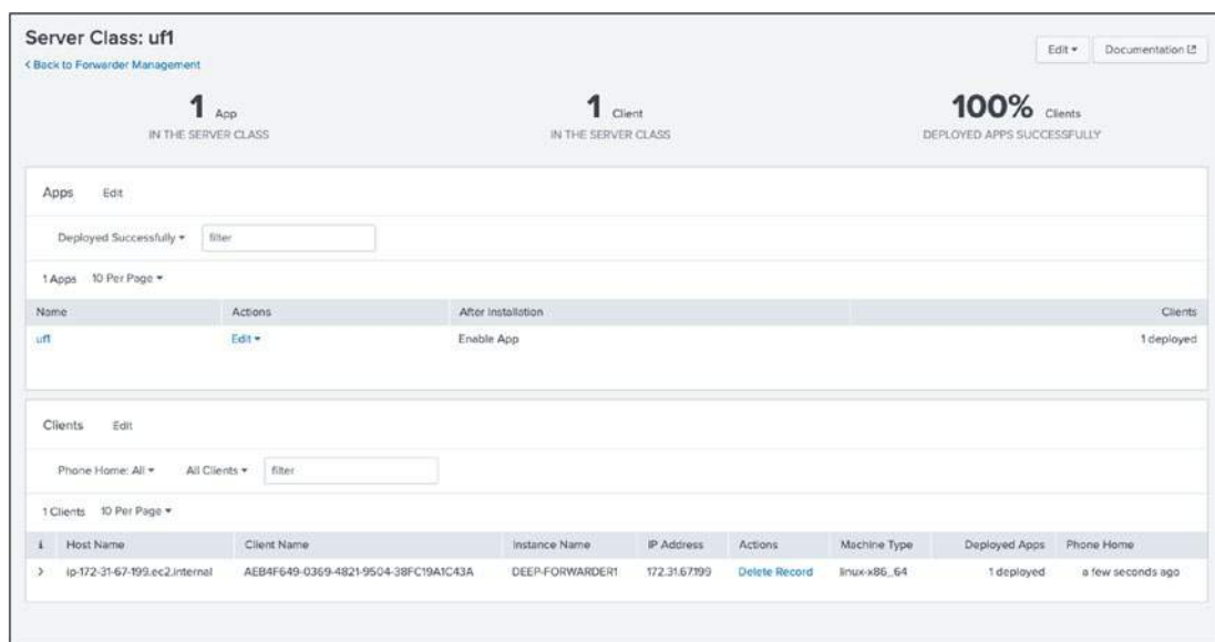
Figure 18-15. Server Class:ufl
