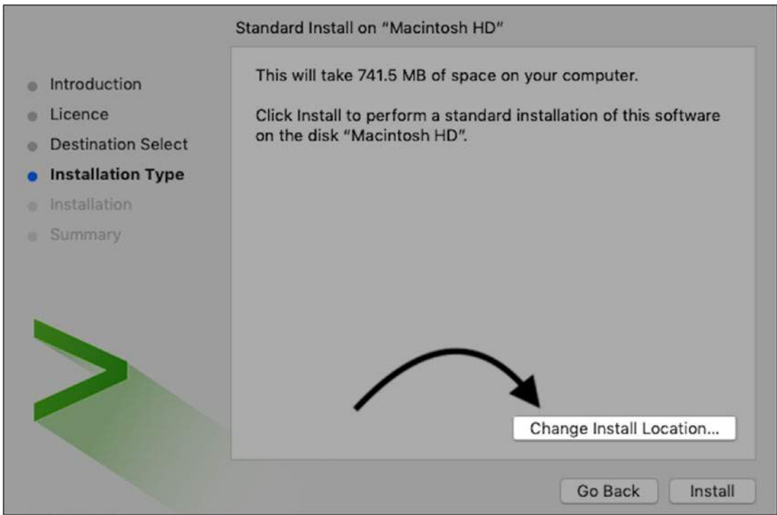
Figure 1-4. Installing Splunk
