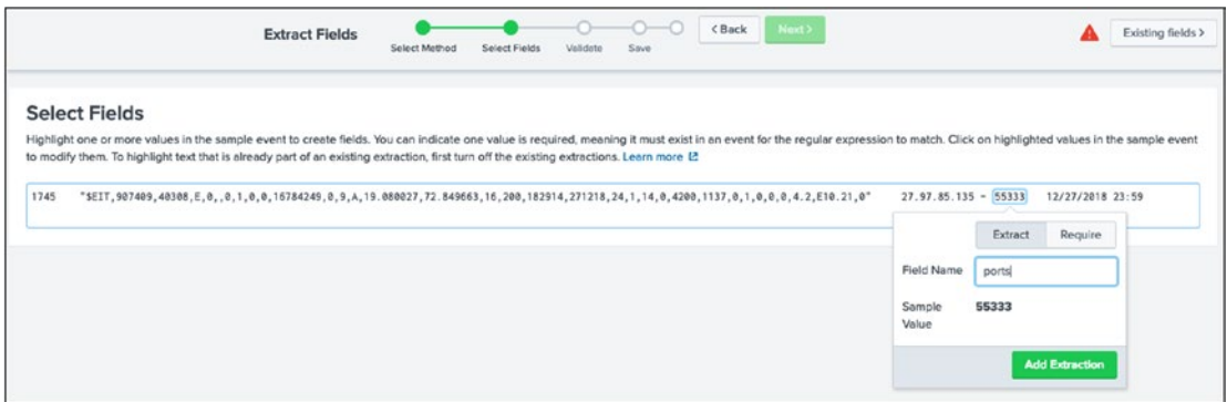
Figure 3-1. Regular Expression Field Extraction
