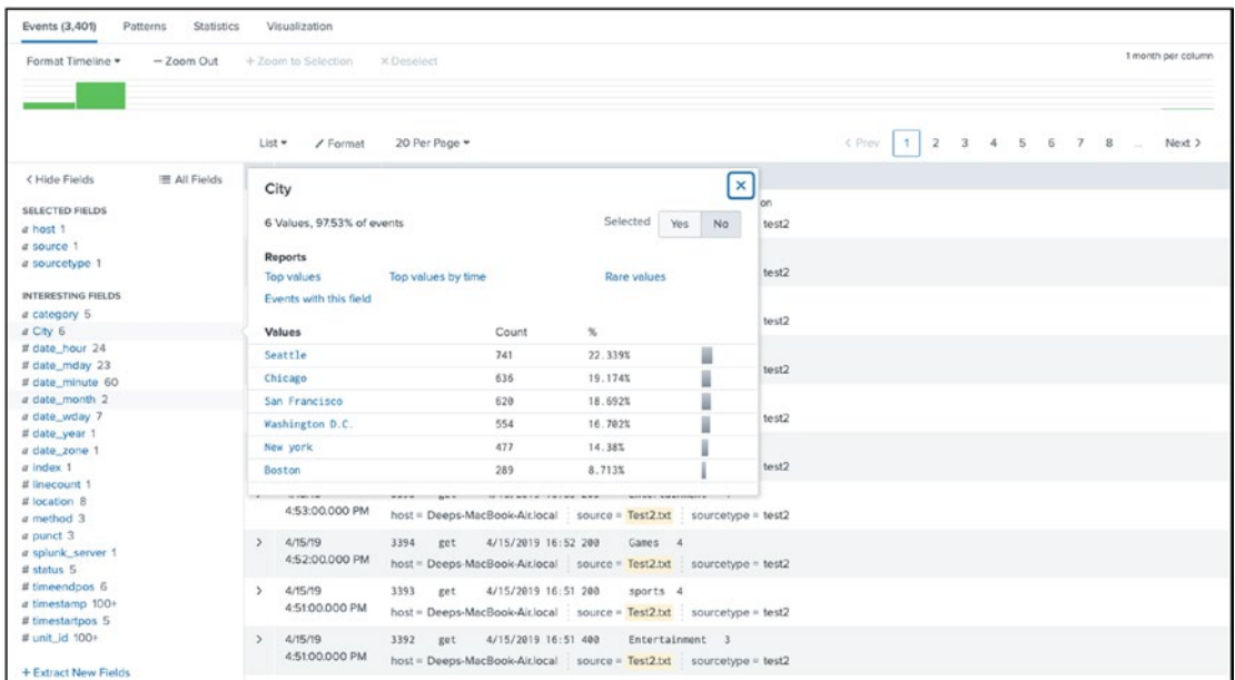
Figure 4-6. Splunk lookup
