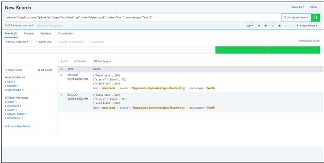
Figure 10-4. Scripted input:1.py
