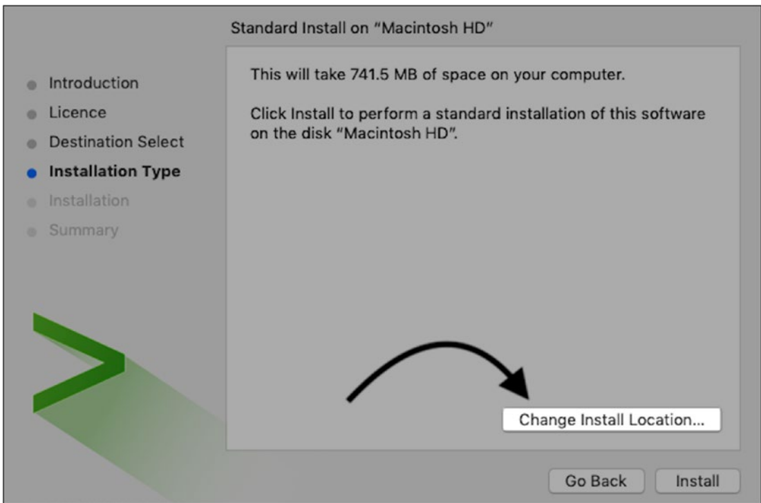
Figure 1-4. Installing Splunk
