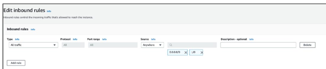
Figure 18-3. Security Group:Main
