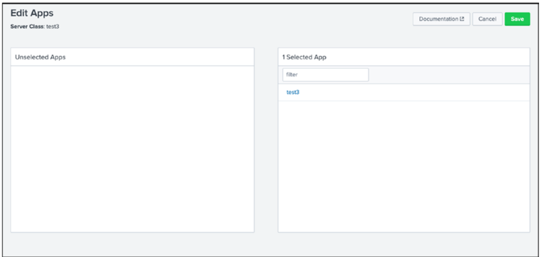
Figure 15-1. Forwarder Management
