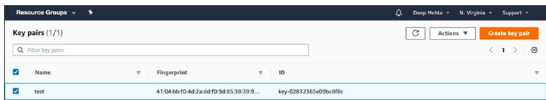
Figure 18-2. Key Pair:Test
