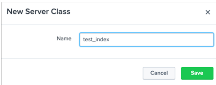
Figure 15-3. Server Class:test_index
