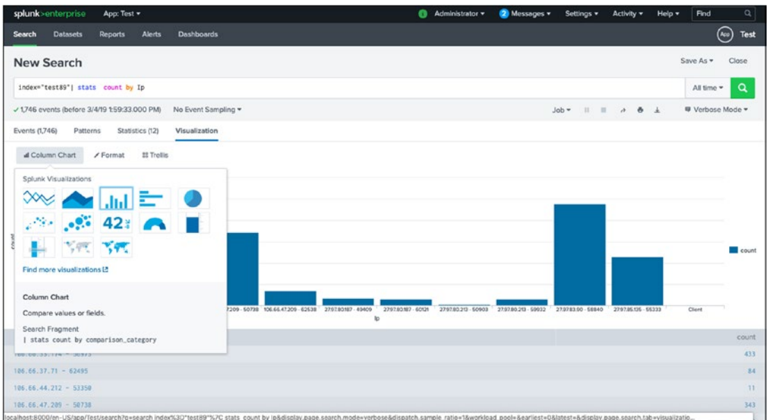
Figure 4-10. Splunk visualization
