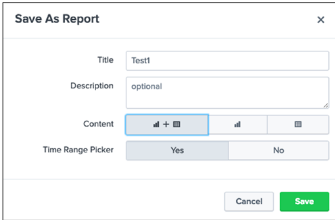
Figure 4-11. Splunk report
