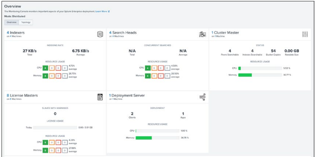
Figure 14-5. Monitoring Console:Deployment
