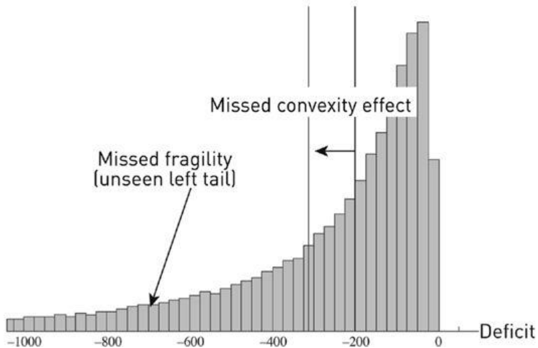
FIGURE 37. Nonlinear transformations allow the detection of both model convexity bias and fragility. Illustration of the example: histogram from Monte Carlo simulation of government deficit as a left-tailed random variable simply as a result of randomizing unemployment, of which it is a concave function. The method of point estimate would assume a Dirac stick at -200 , thus underestimating both the expected deficit ( -312 ) and the tail fragility of it. (From Taleb and Douady, 2012).
